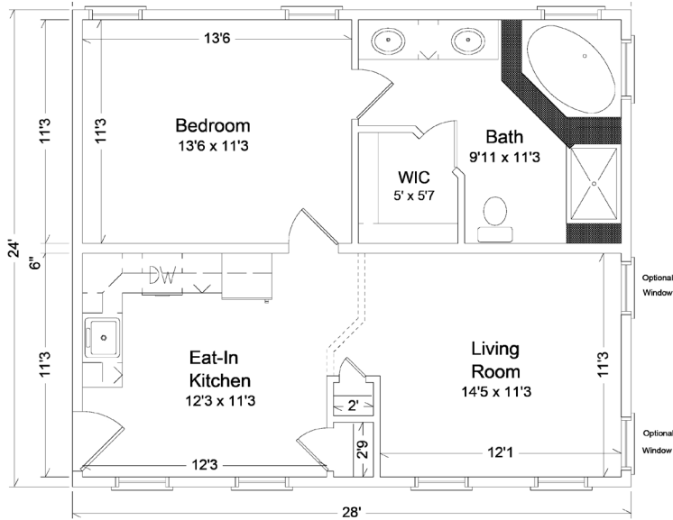
In-Law Suite #1- 672 Sq Ft
